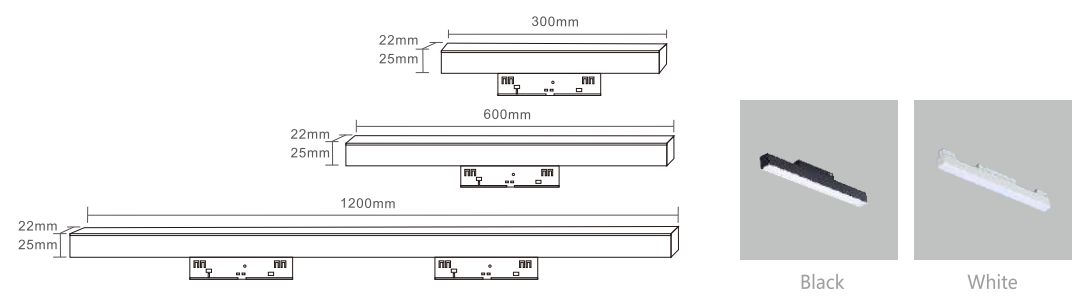
磁吸泛光灯系列 48V Magnetic Flood Light Series
