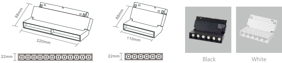
磁吸折叠灯系列 48V Magnetic Folding Light Series
