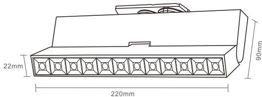
折叠格栅轨道灯系列 220V LED Track Light Series
